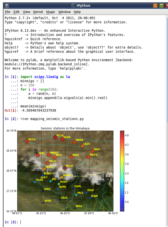
Figure 1: The IPython Qt console: a lightweight terminal for scientific exploration, with code, results and graphics in a soingle environment.
